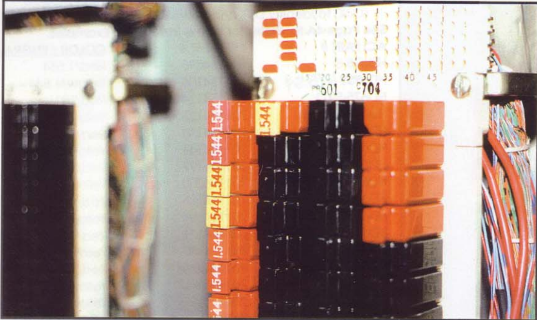
3A MODULES (COILS) WITH 1.544 I.D. CAPS & TEST POINT ACCESS PLUGS INSTALLED
