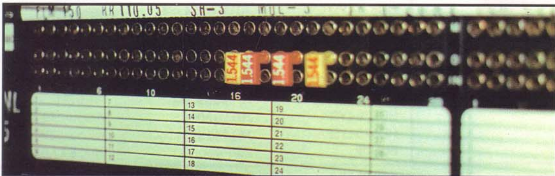
BANTAM DSX PANEL WITH I.D. PLUGS & 1.544 I.D. CAPS INSTALLED
