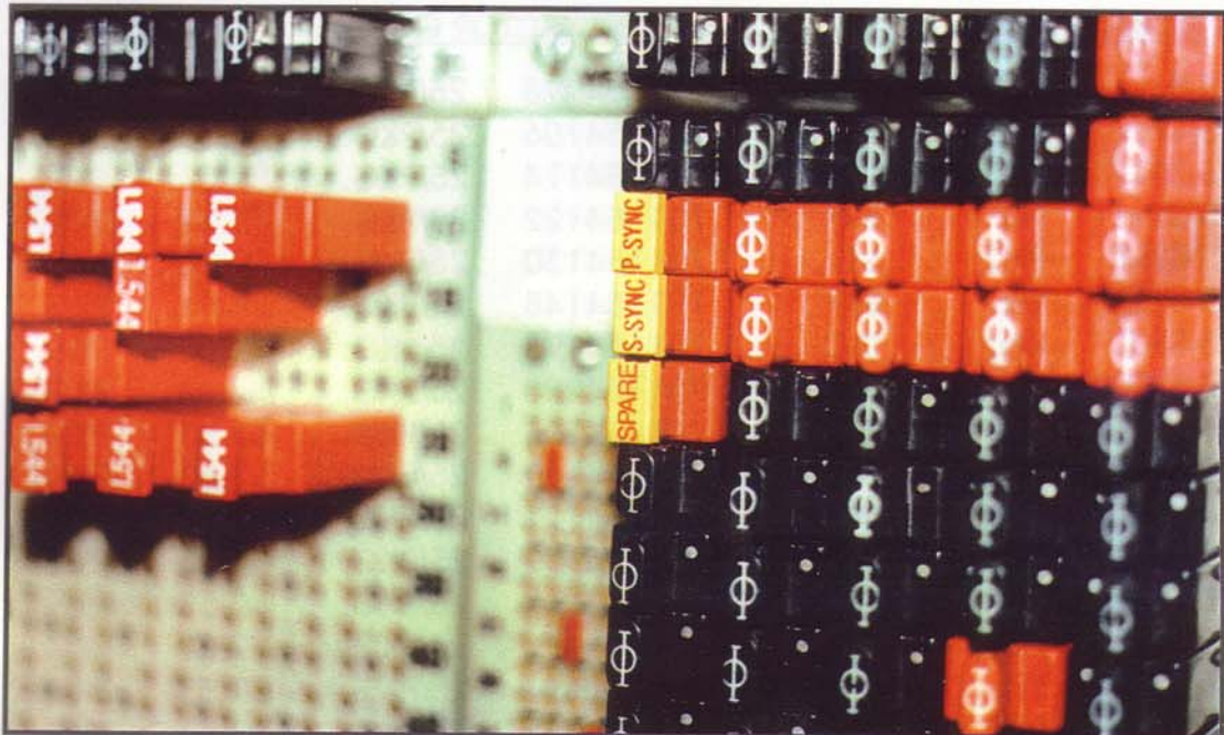
4C MODULES (COILS) WITH P-SYNC, S-SYNC & SPARE I.D. CAPS & TEST POINT ACCESS PLUGS INSTALLED
