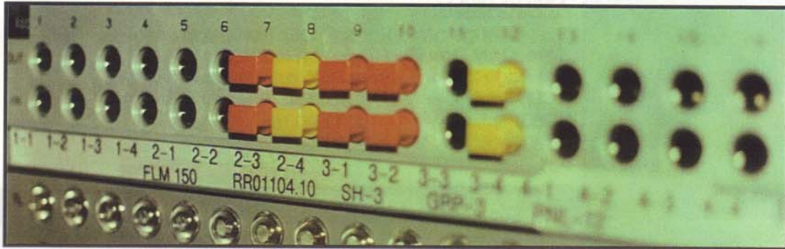
310 DSX PANEL WITH I.D. PLUGS AND NO I.D. CAPS INSTALLED
