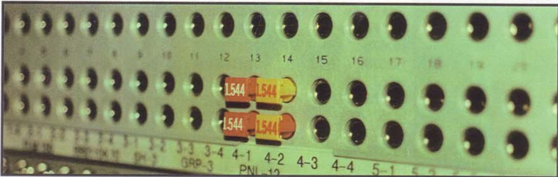
310 DSX PANEL WITH I.D. PLUGS & 1.544 I.D. CAPS INSTALLED
