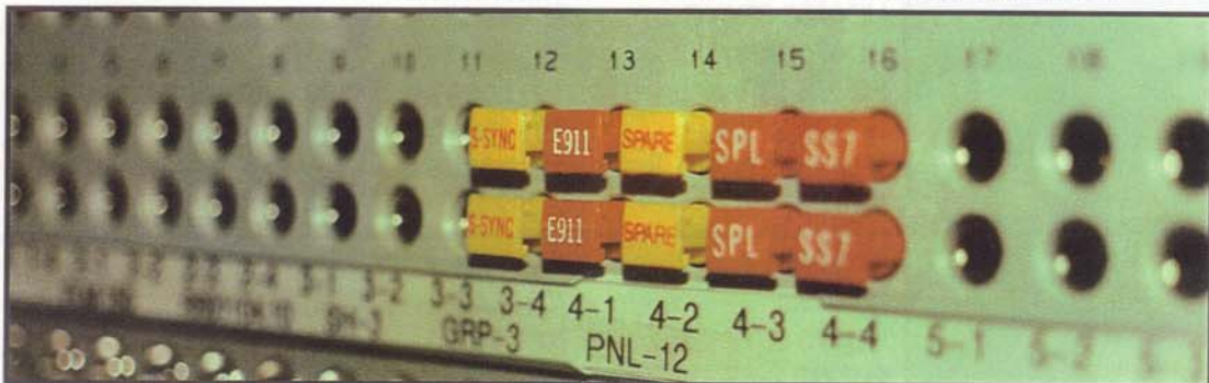
310 DSX PANEL WITH I.D. PLUGS AND VARIOUS I.D. CAPS INSTALLED
