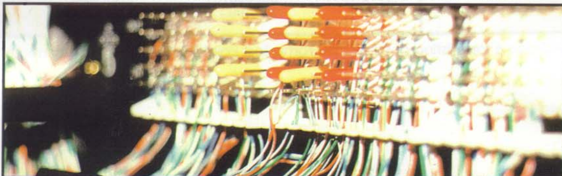
WIRE WRAP INSULATORS ON REAR OF BANTAM DSX PANEL INSTALLED
