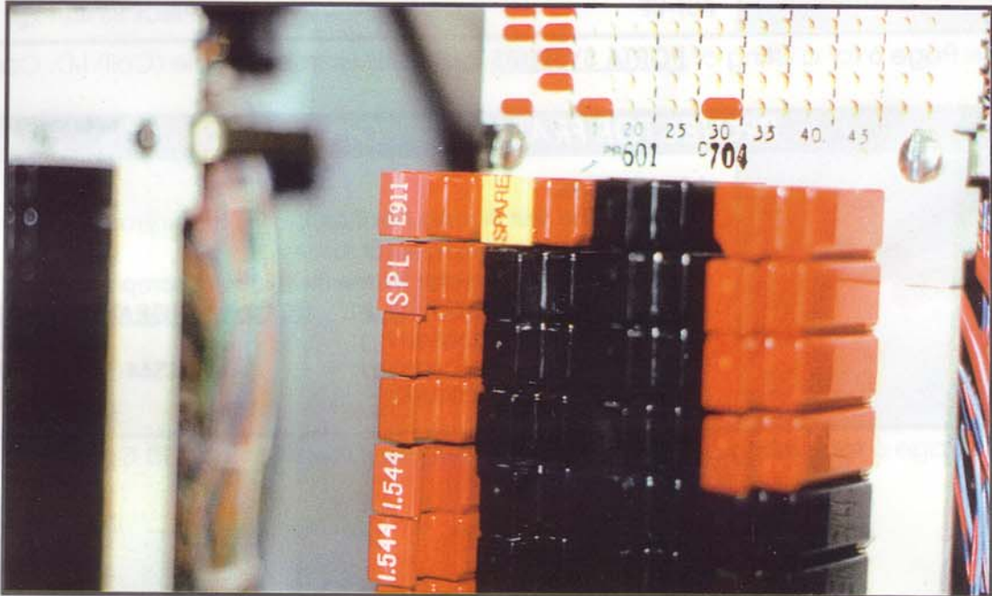
3A MODULES (COILS) WITH E911, SPL, SPARE I.D. CAPS & TEST POINT ACCESS PLUGS INSTALLED
