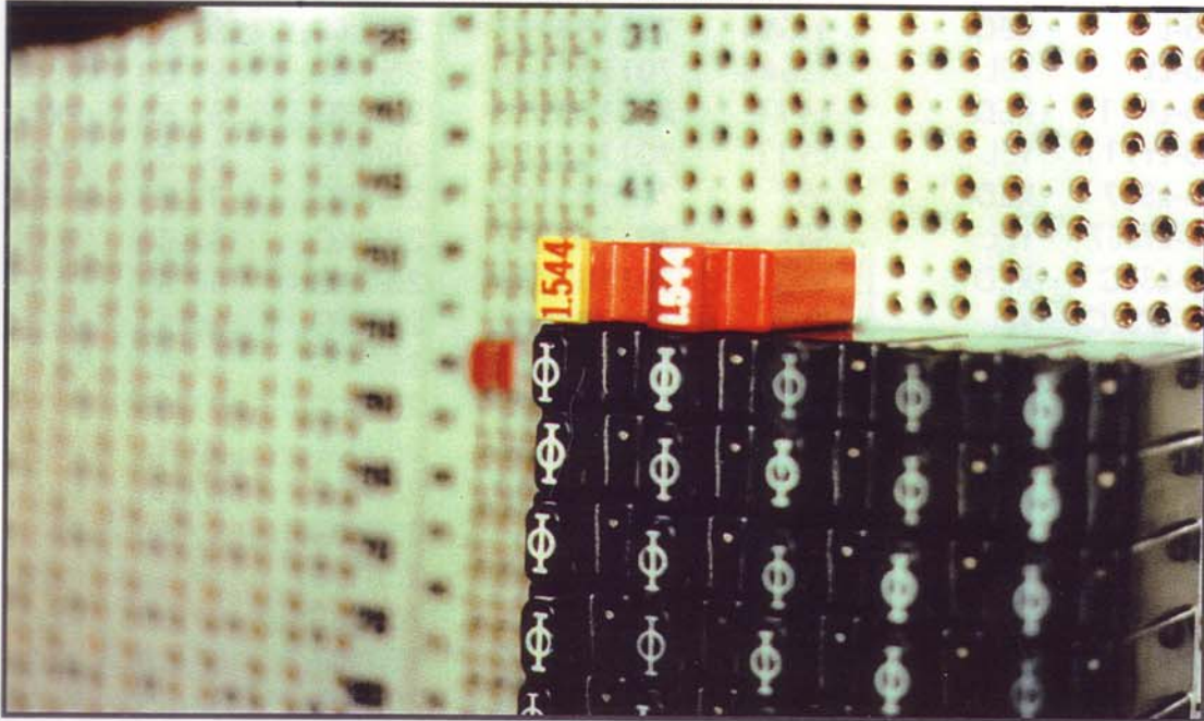
4C MODULES (COILS) WITH 1.544 I.D. CAPS & TEST POINT ACCESS PLUGS INSTALLED
